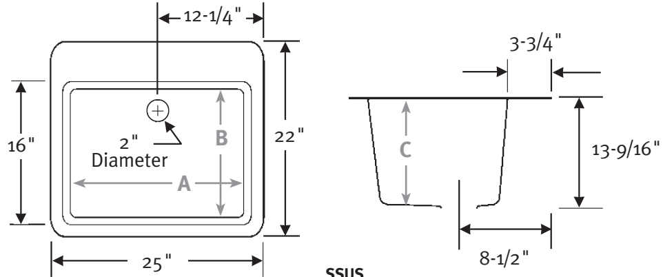
SSUS 25" W x 22" D (635 mm x 559 mm) A 21-1/2", B 16", C 13-9/16" Capacity: 17-1/2 gallons
